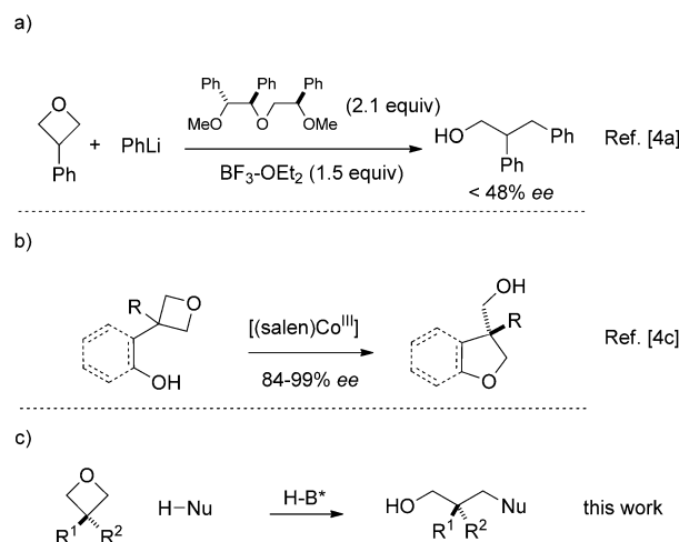
Scheme 1. Enantioselective desymmetrization of 3-substituted oxetanes. a) First and only intermolecular example (noncatalytic, low ee values). [4a] b) First intramolecular example (catalytic, good ee values). [4c] c) First intermolecular catalytic example (good ee values).
