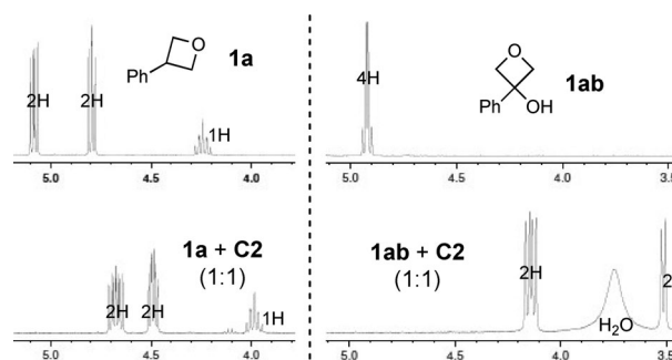
Figure 2. NMR observation of the substrate–catalyst interaction. [14] Values on the horizontal axes: \delta(^1\text{H}) [ppm].
